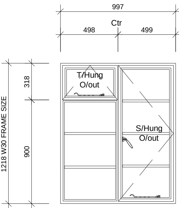
WINDOW NUMBERS/LOCATION: W1.04, W1.05, W1.06, W1.07 FRAME TYPE W30 SECTIONS
