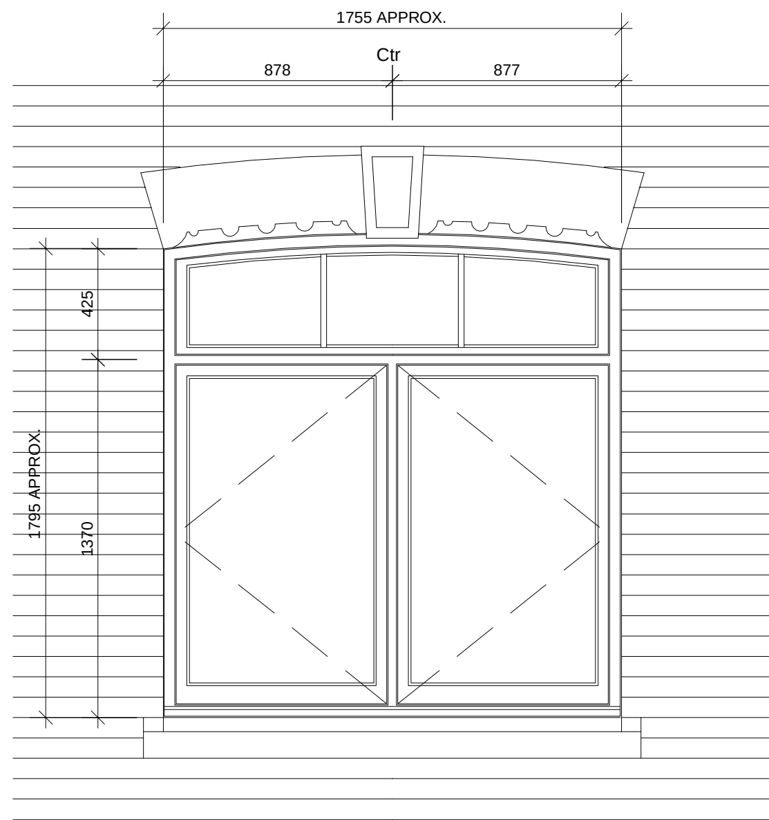
WINDOW NUMBERS: W1.01, W1.02, W1.03 TIMBER CASEMENT (EGRESS)
