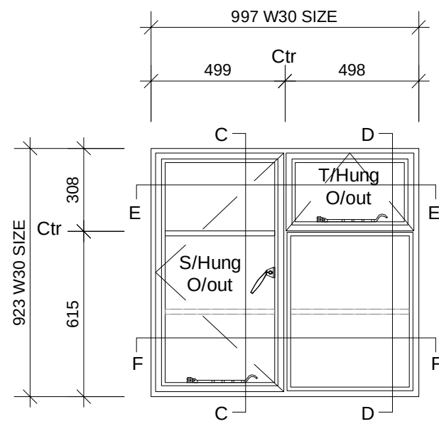
WINDOW NUMBERS/LOCATION: W0.03 FRAME TYPE W30 SECTIONS
