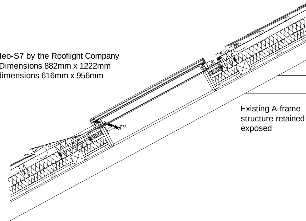
ROOFLIGHT SECTION
