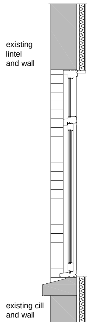
TIMBER CASEMENT SECTION
