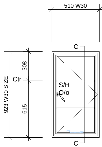
WINDOW NUMBERS/LOCATION: W0.04 FRAME TYPE W30 SECTIONS
