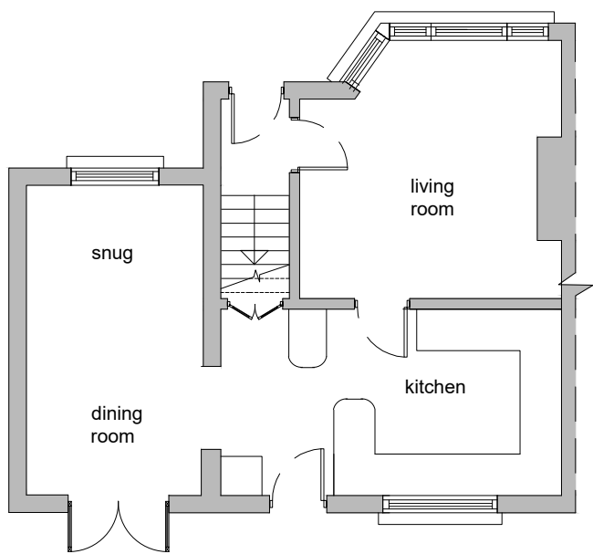
EXISTING GROUND FLOOR
