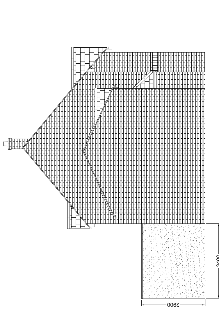
Proposed Side Elevation - East Facing Scale 1:100 @A3
