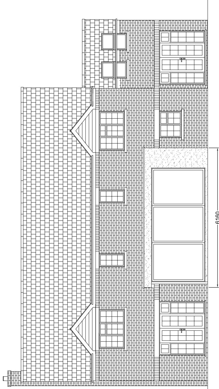
Proposed Rear Elevation Scale 1:100 @A3
