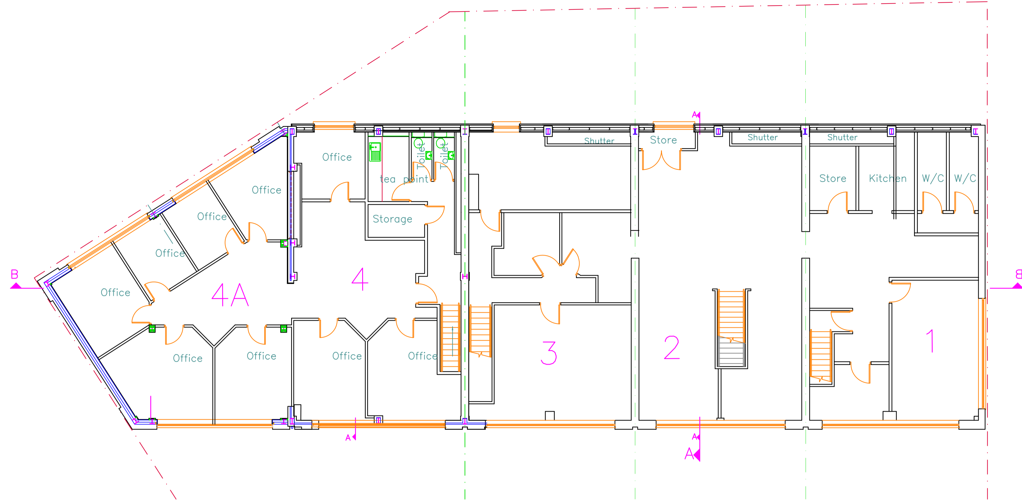
EXISTING FIRST FLOOR LAYOUT
