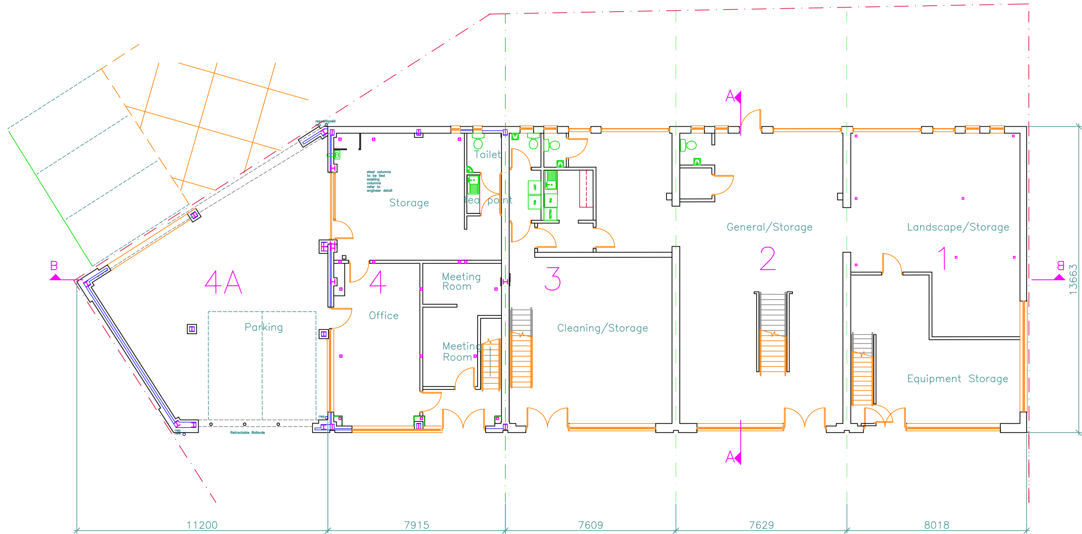
EXISTING GROUND FLOOR LAYOUT
