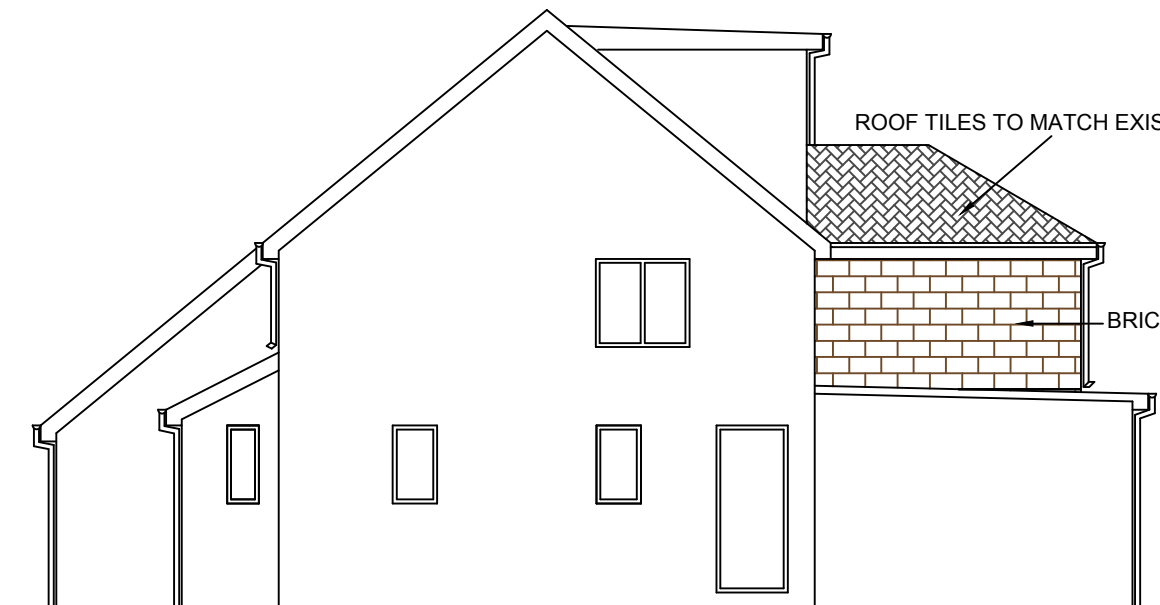
RIGHT SIDE ELEVATION PROPOSED
