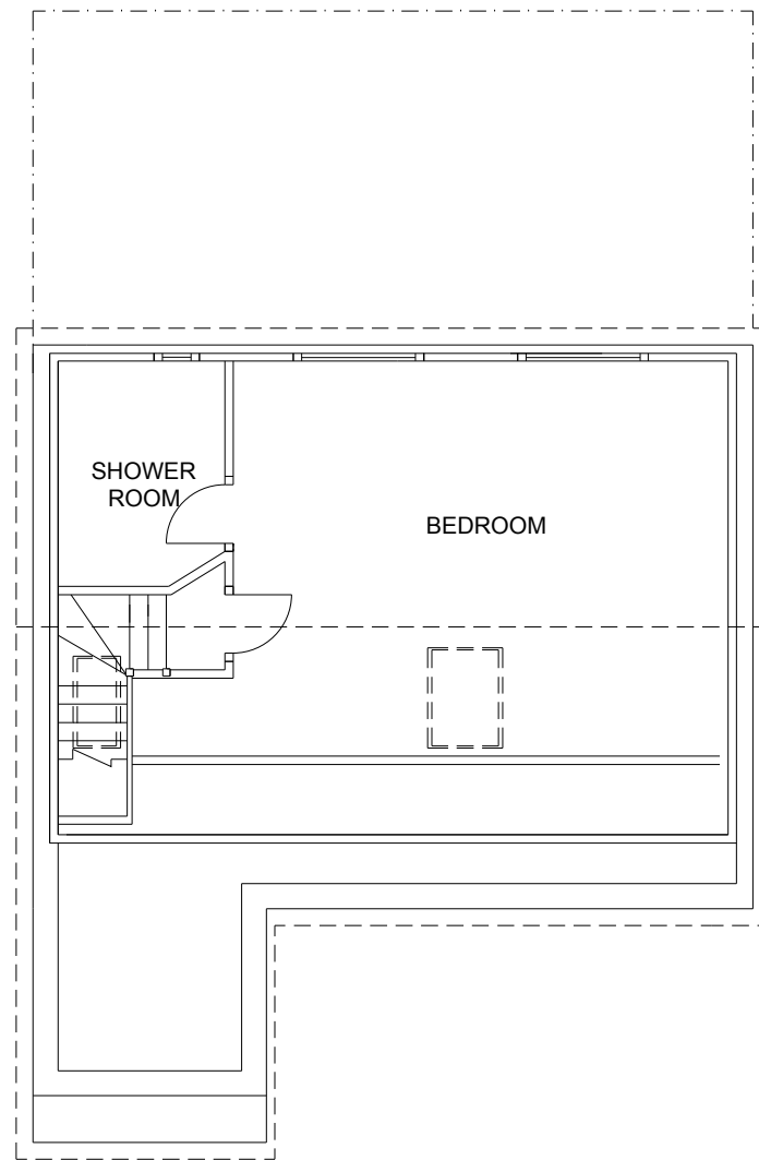
LOFT FLOOR PLAN EXISTING
