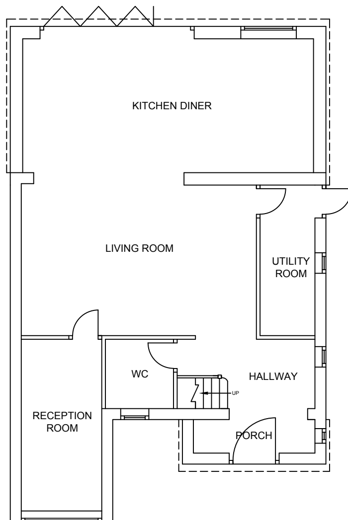
GROUND FLOOR PLAN EXISTING
