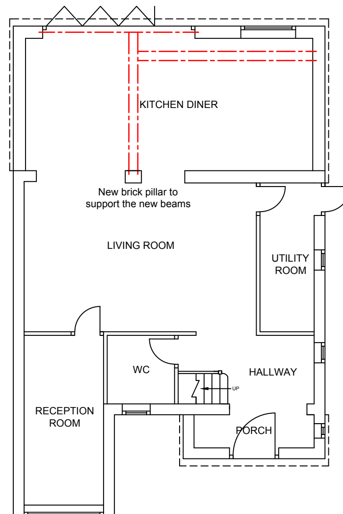
GROUND FLOOR PLAN PROPOSED
