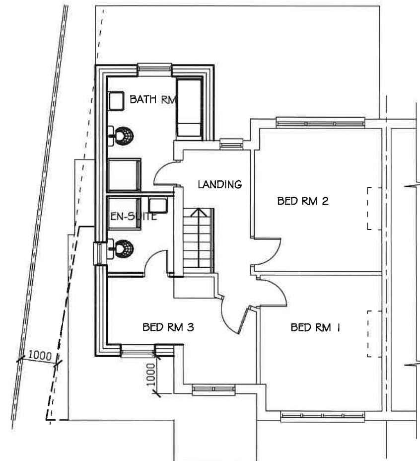
PROPOSED FIRST FLOOR PLAN SCALE= 1:100
