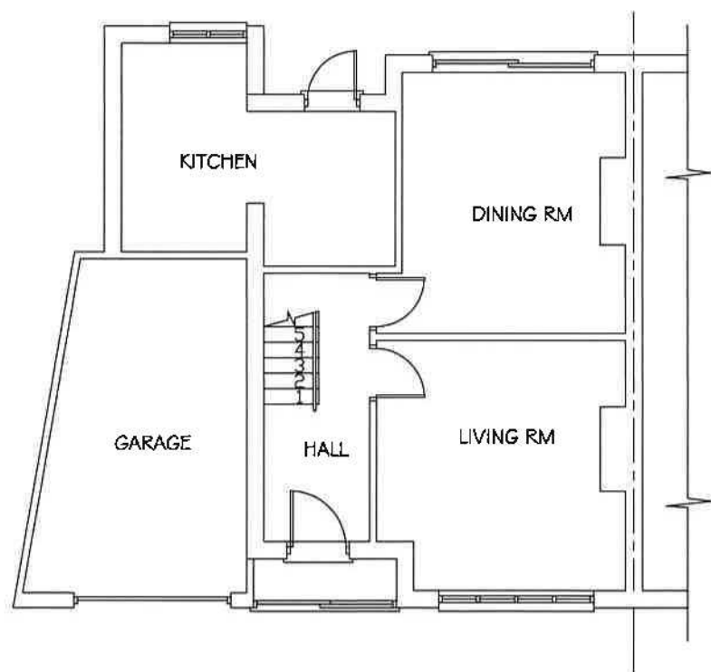
EXISTING GROUND FLOOR PLAN SCALE= 1:100
