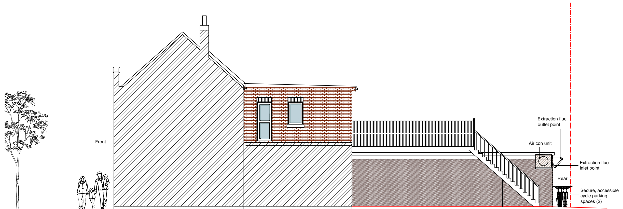
PROPOSED B-B SIDE ELEVATION
