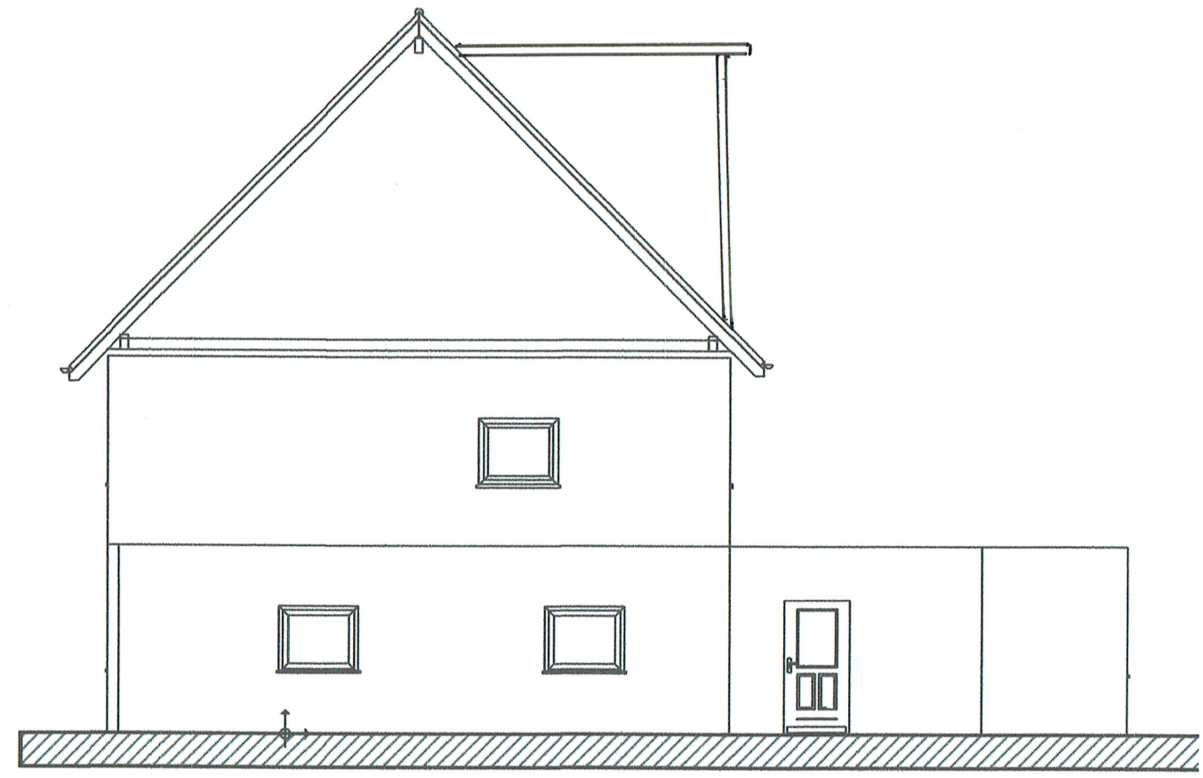
REAR ELEVATION
