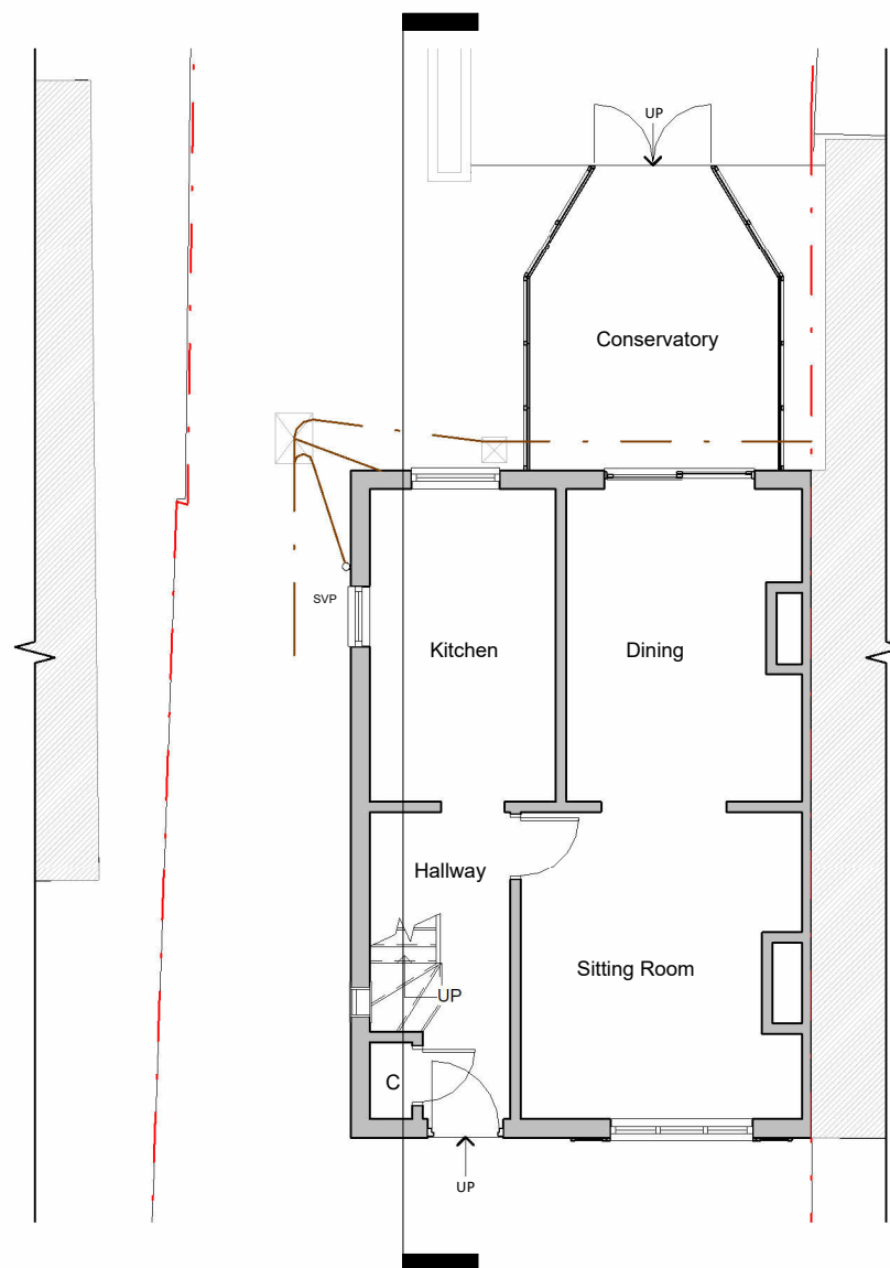
Ground floor 1 : 100
