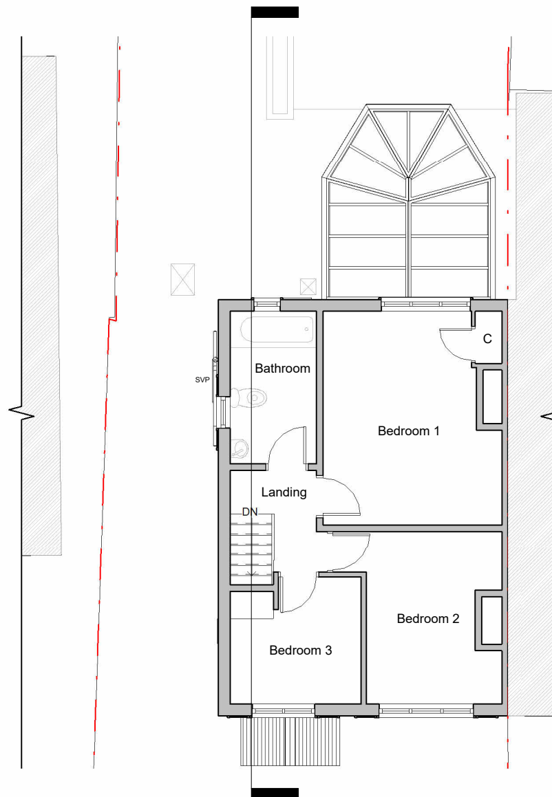
First floor 1 : 100
