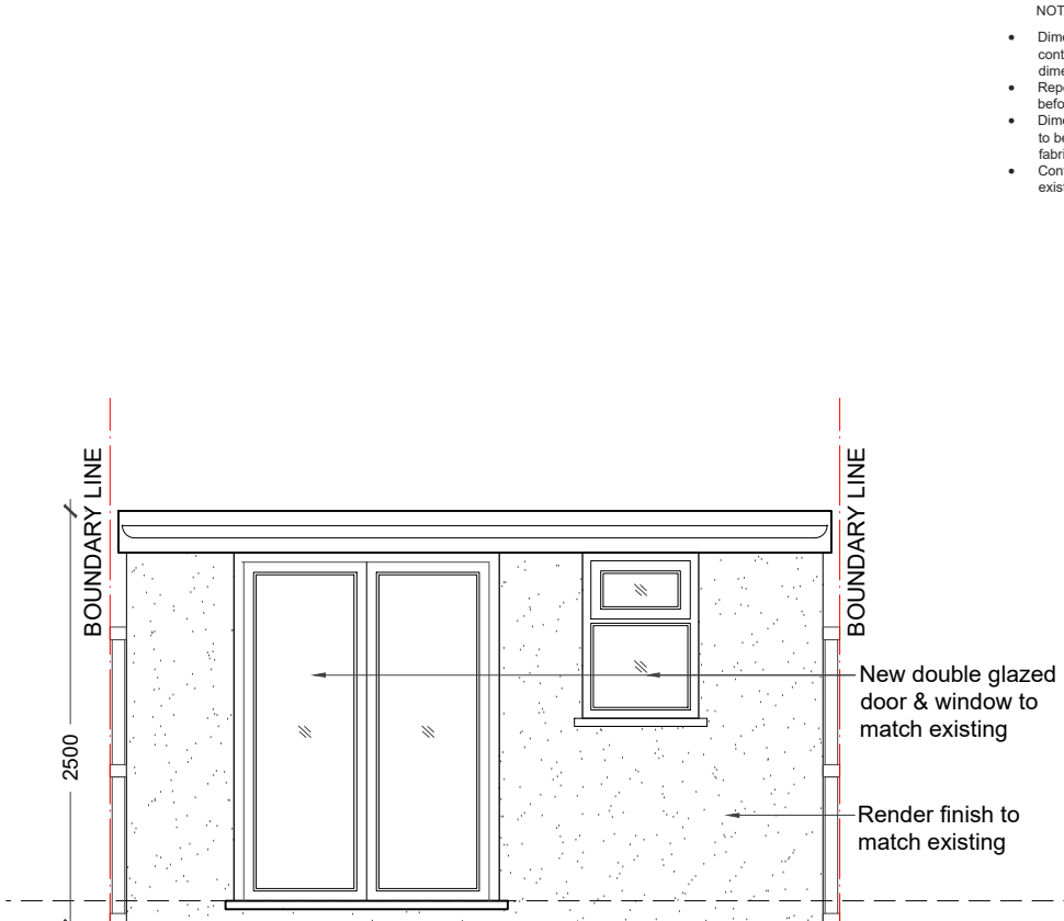
03 - FRONT ELEVATION
