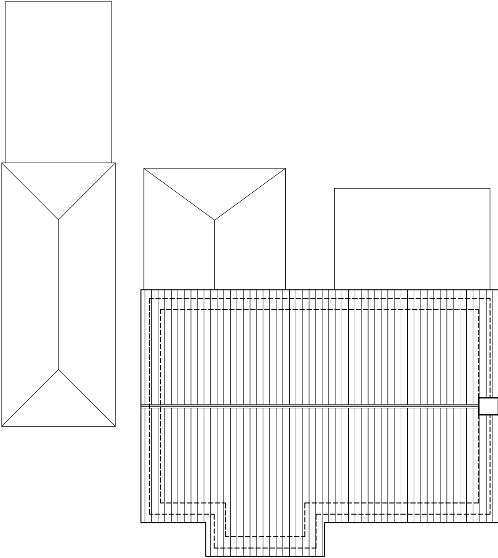
ROOF PLAN
