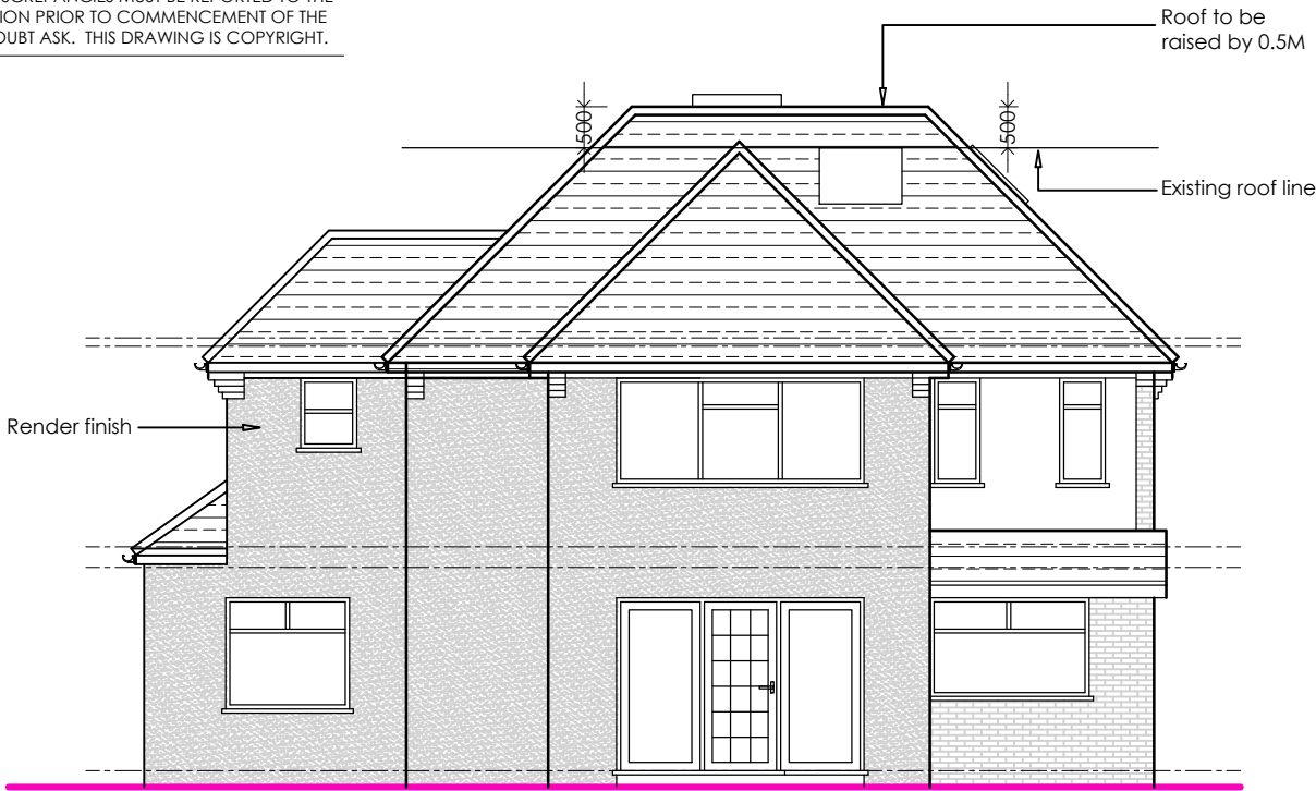
FRONT ELEVATION
