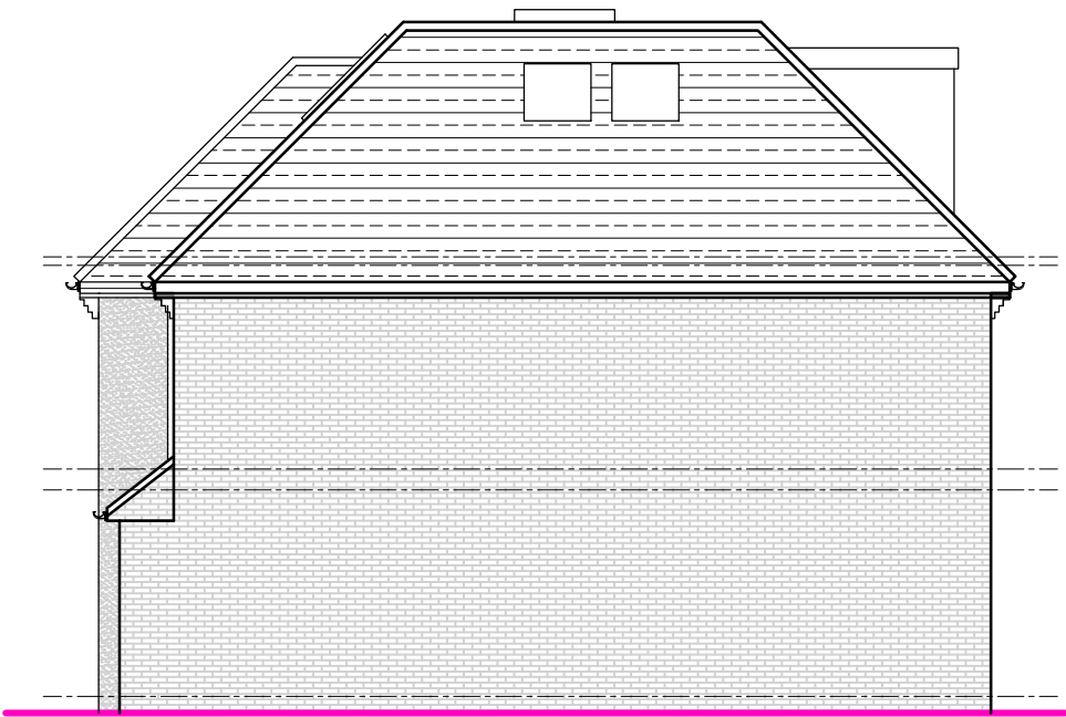
SIDE ELEVATION FACING No. 50
