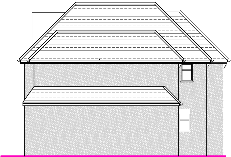
SIDE ELEVATION FACING No. 54
