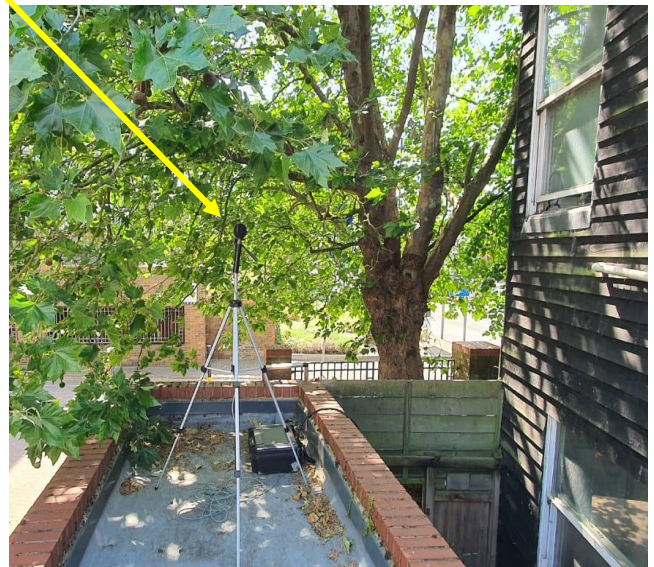
Figure 5.2.1 – Measurement Location
