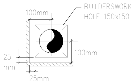
SETTING OUT FOR Ø110mm SVP/WVP/SP (DP) LOCATED IN A 90° CORNER
