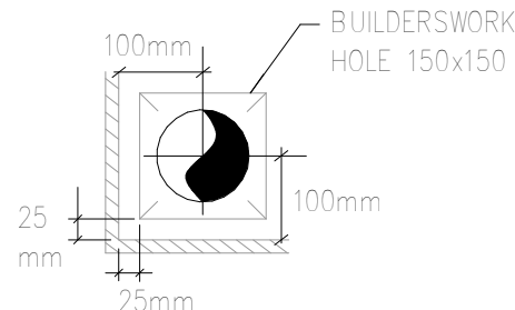
SETTING OUT FOR Ø110mm SVP/WVP/SP (DP) LOCATED IN A 90° CORNER
