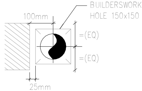
SETTING OUT FOR Ø110mm SVP/WVP/SP (DP) ADJACENT TO STRUCTURAL COLUMN
