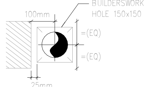
SETTING OUT FOR Ø110mm SVP/WVP/SP (DP) ADJACENT TO STRUCTURAL COLUMN
