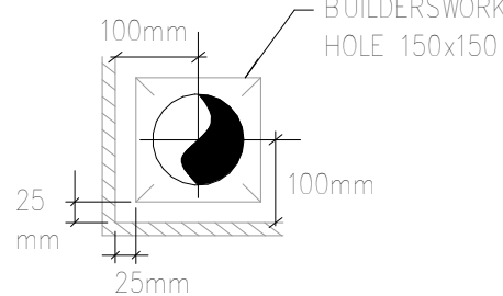
SETTING OUT FOR Ø110mm SVP/WVP/SP (DP) LOCATED IN A 90° CORNER
