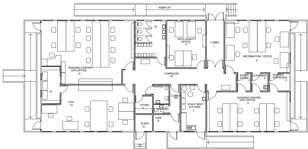
OLD CRECHE GROUND FLOOR GROSS INT AREA = 321.6 m sq
