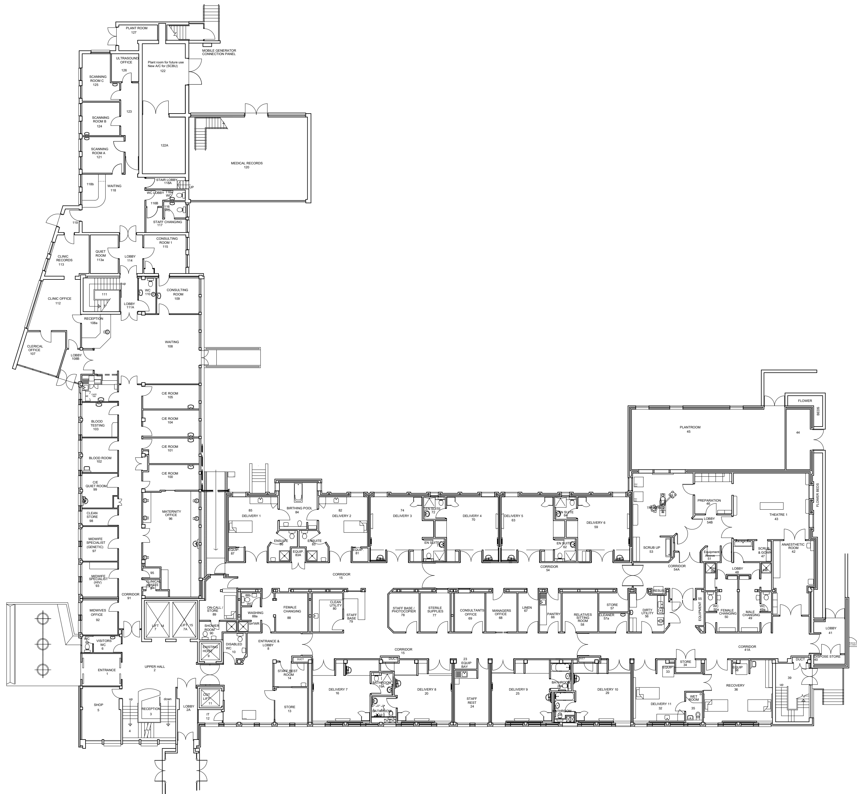
MATERNITY GROUND FLOOR PLAN GROSS INT AREA = 1835.5m sq
