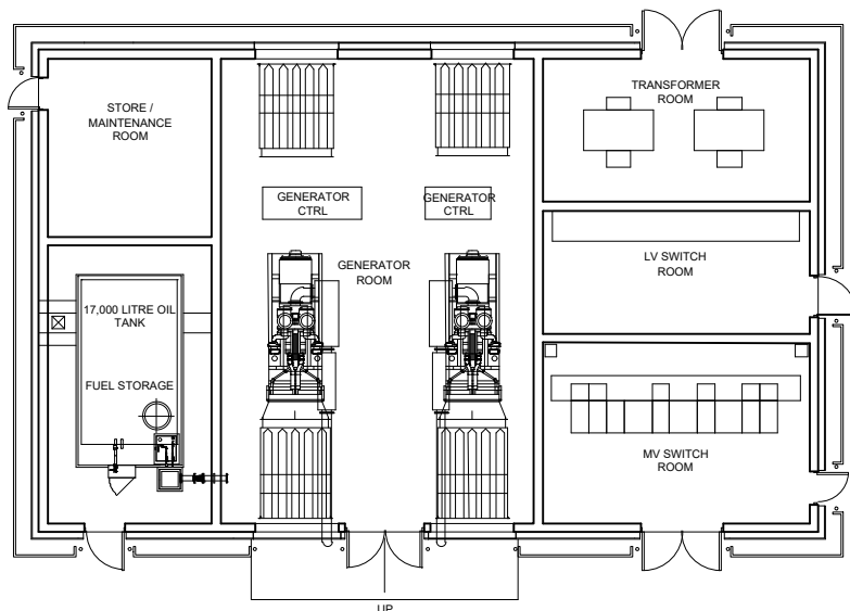
ENERGY CENTRE GROUND FLOOR Gross Internal Area = 210.3 m sq
