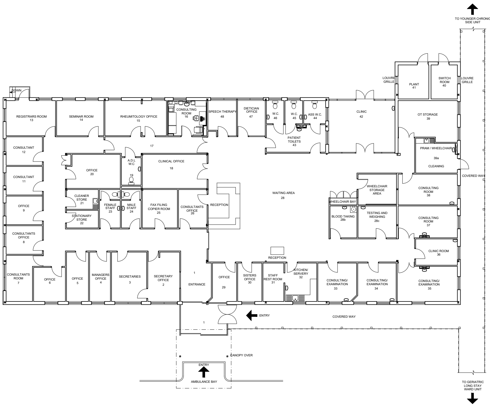
ELDERLEY DAY CARE - GROUND FLOOR PLAN GROSS INT AREA = 769.6 m sq
