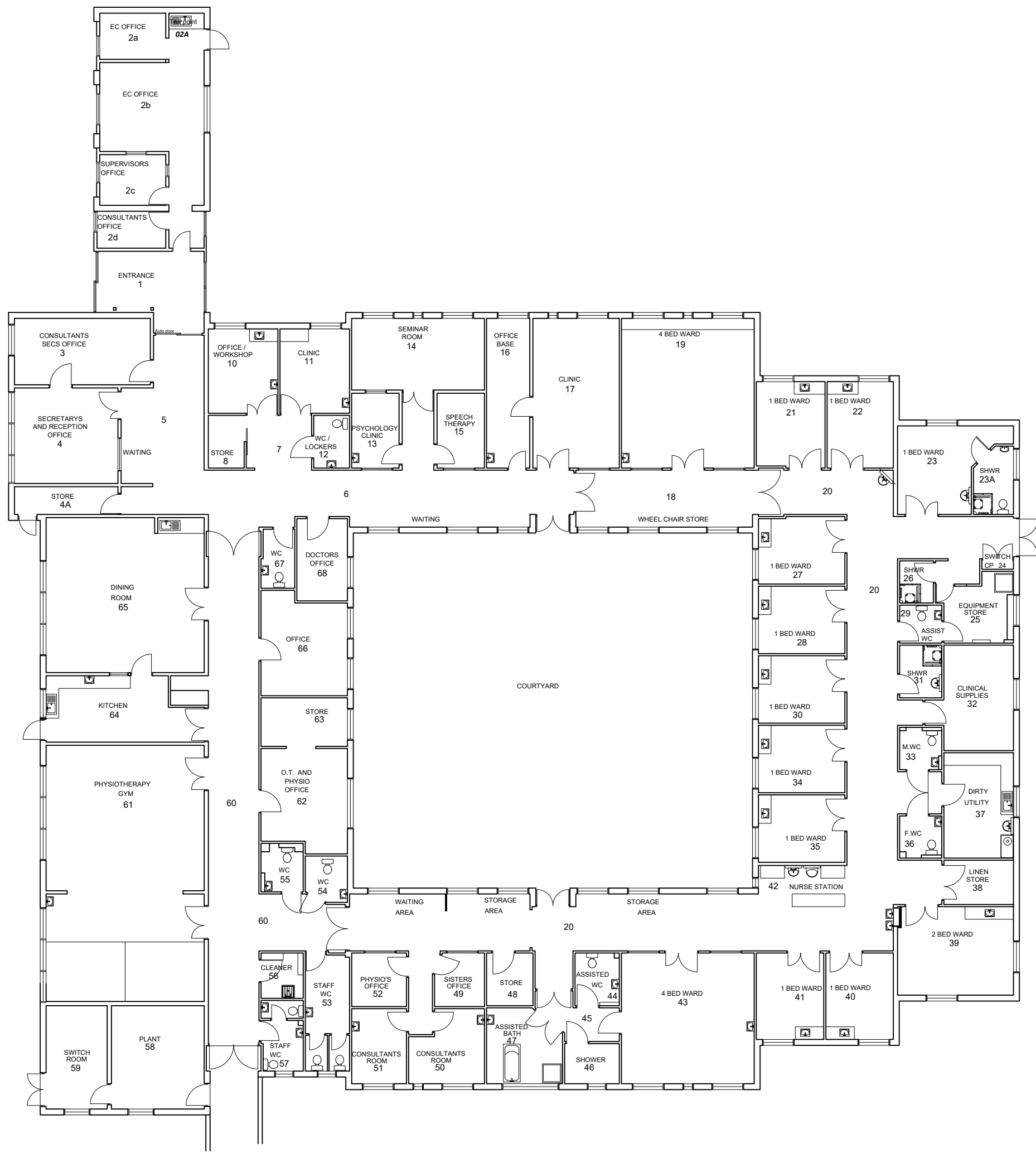
ALDERBOURNE GROUND FLOOR GROSS INTERNAL AREA = 1323.5 m sq
