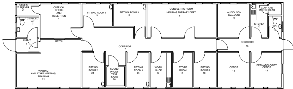
ADULT AUDIOLOGY GROUND FLOOR Gross Internal Area = 178.1 m sq
