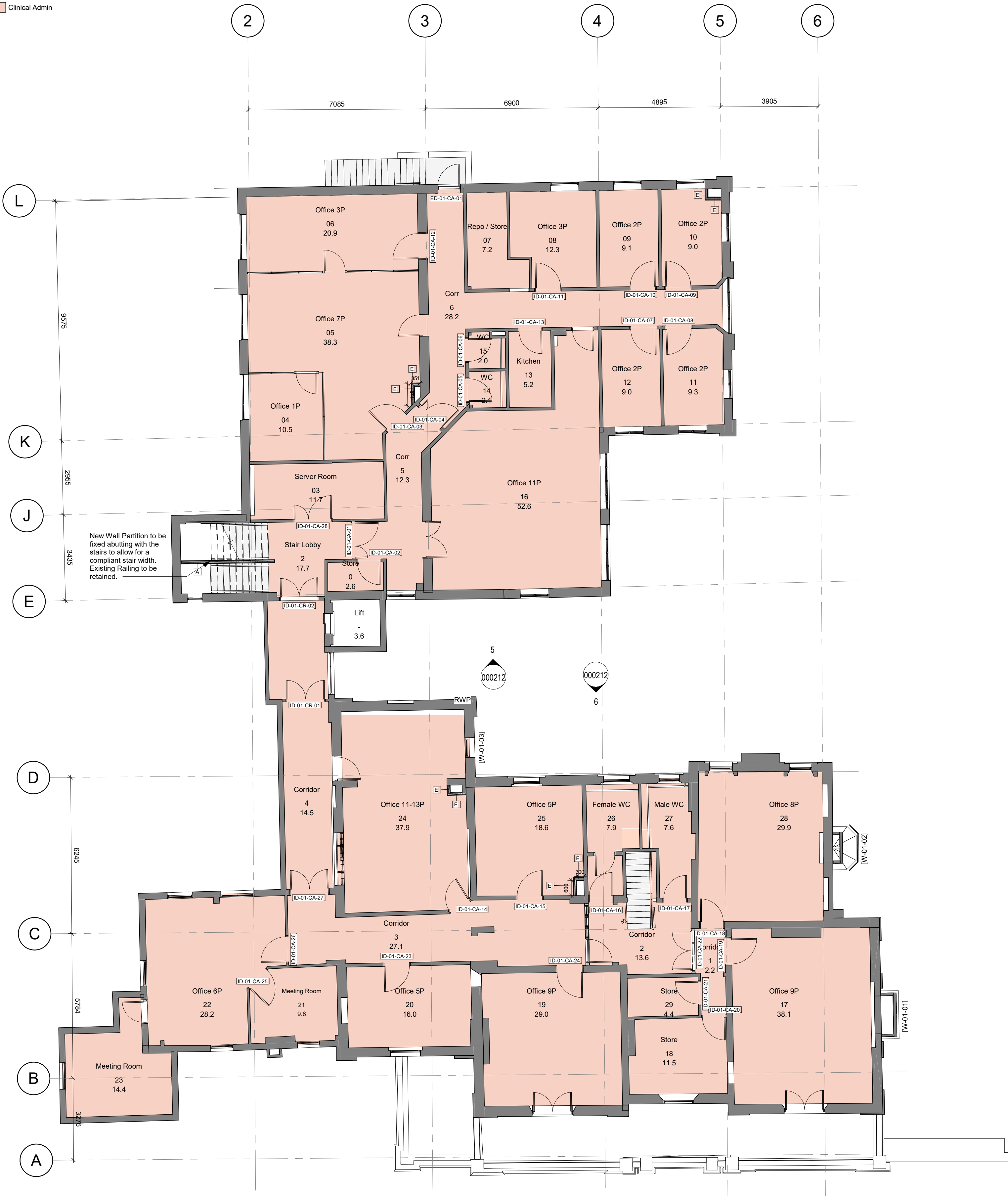
Proposed First Floor Level
