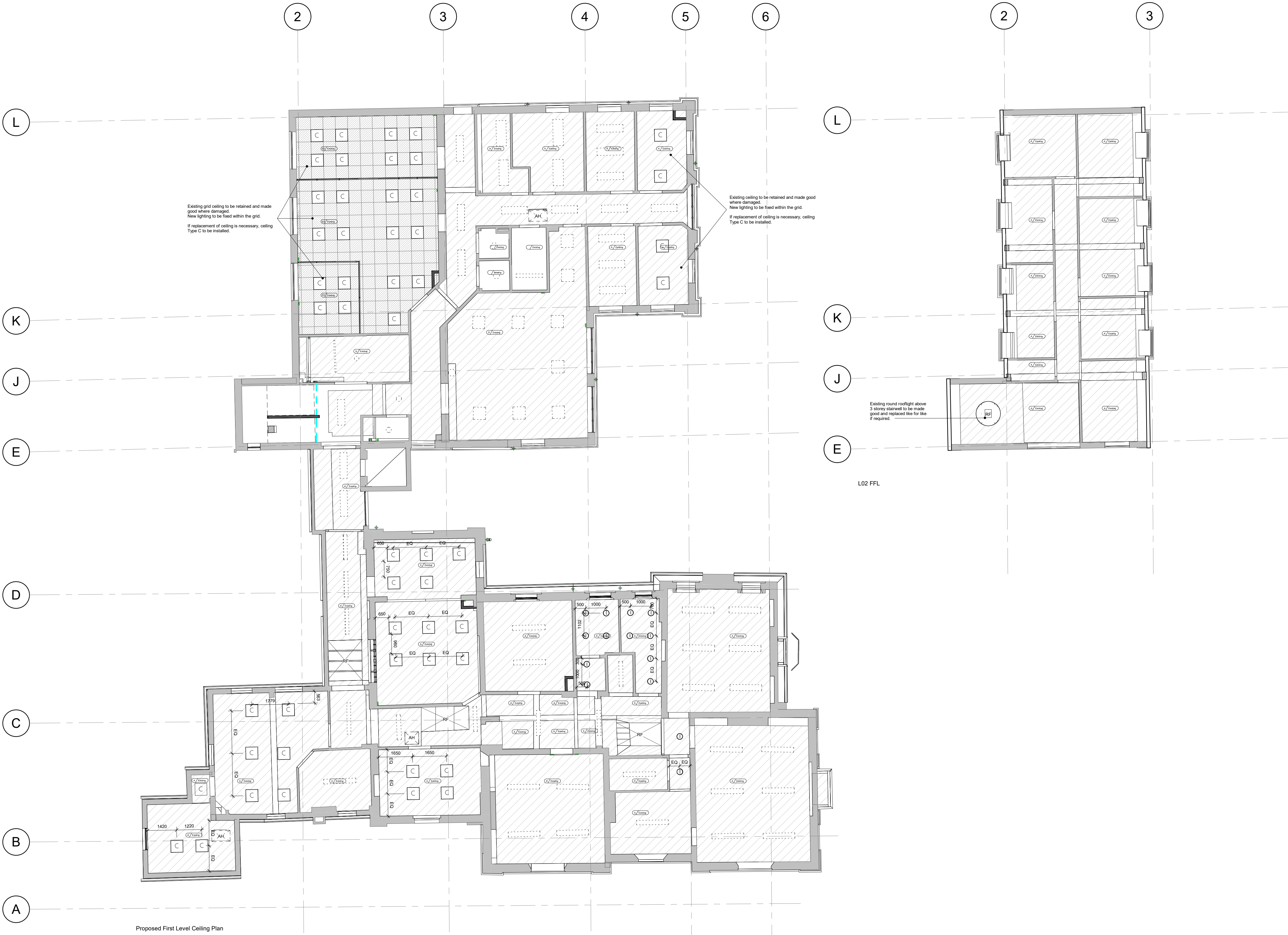
Proposed First Level Ceiling Plan
