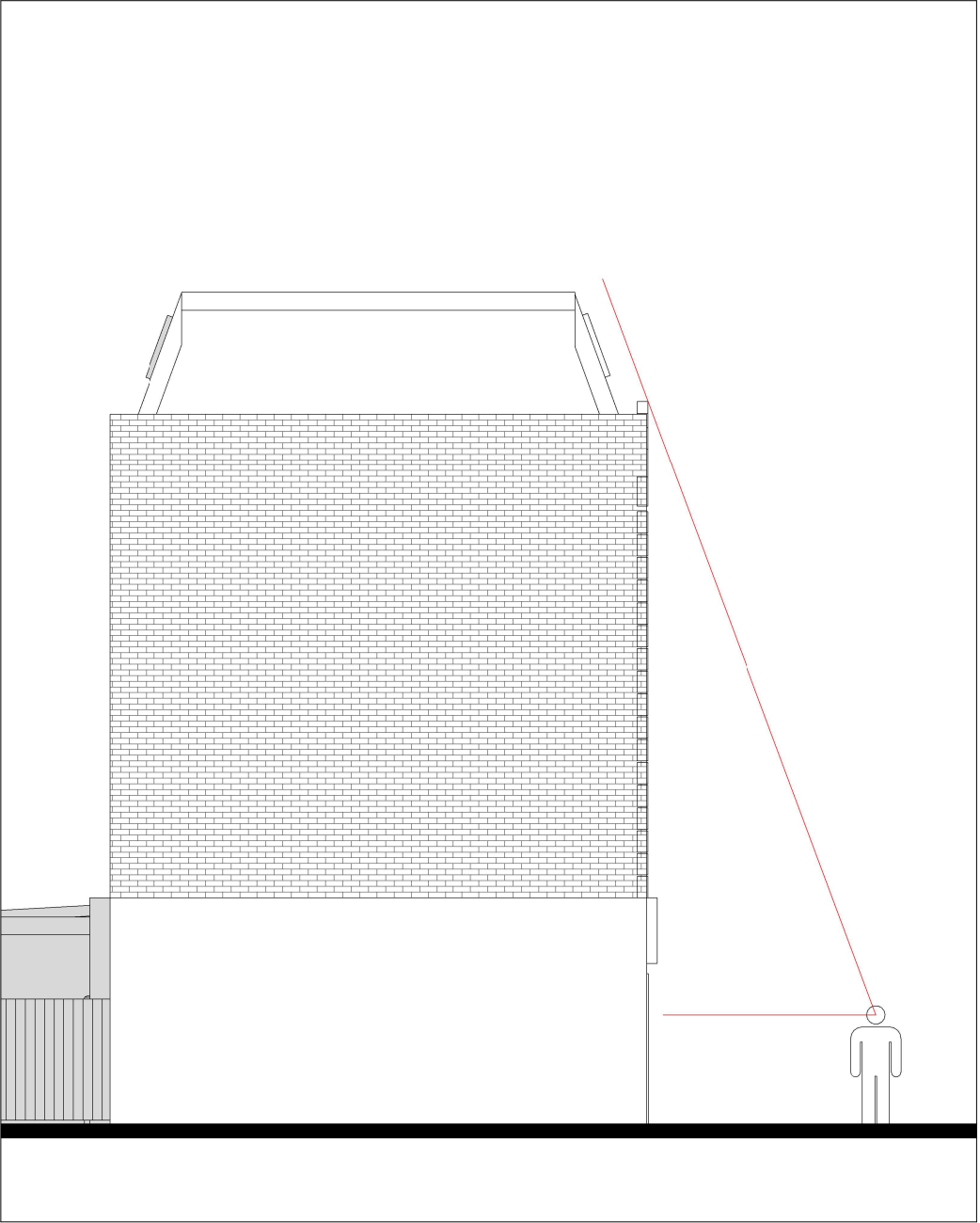
Side Elevation with human view level
