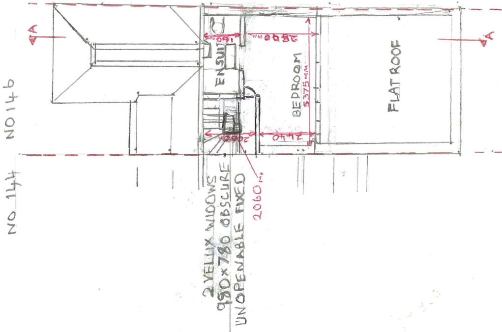
PROPOSED LOFT ROOM PLAN
