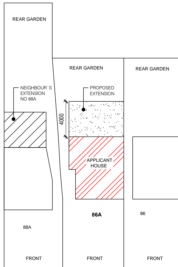
PROPOSED - BLOCK PLAN SCALE 1:250
