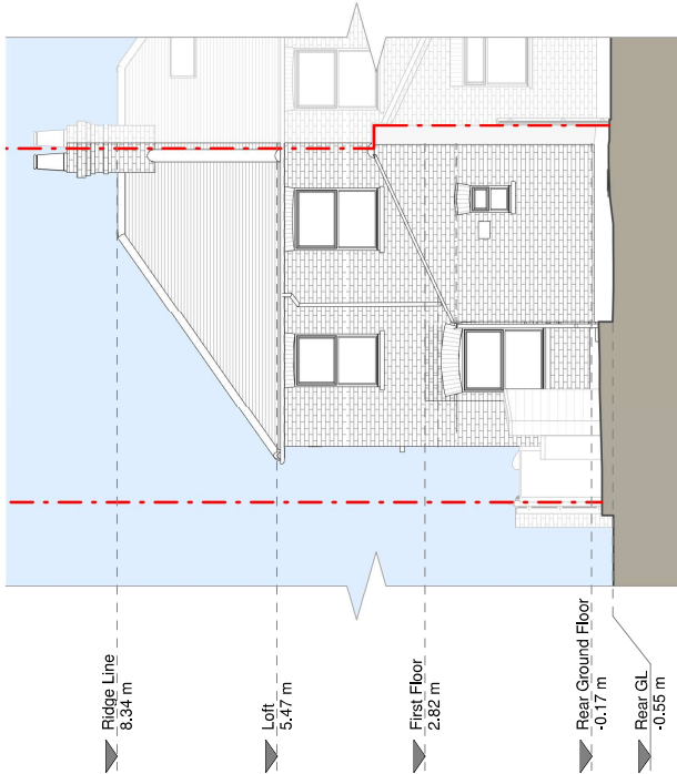
Rear Elevation
