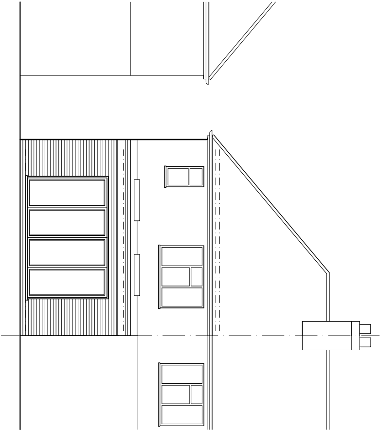
REAR ELEVATION
