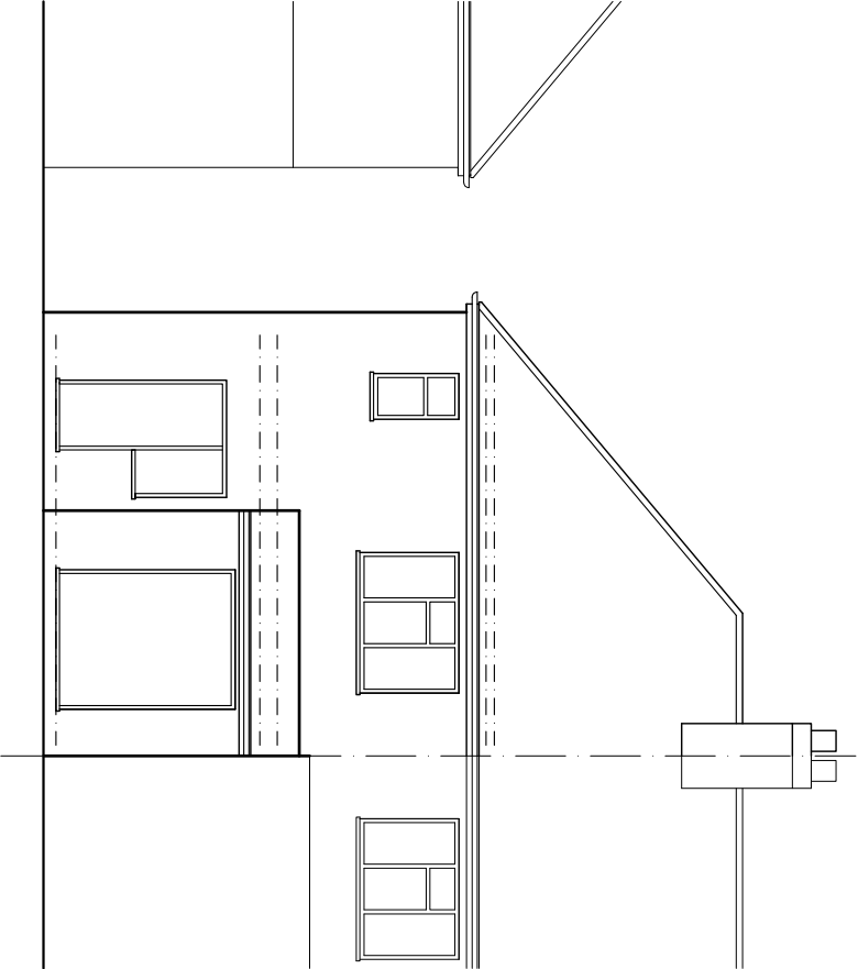
REAR ELEVATION
