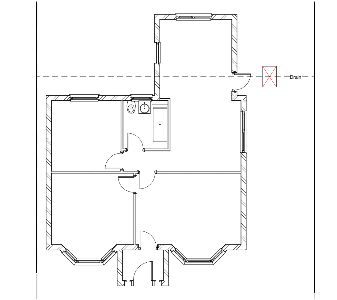
1 Ground Floor 1 : 100
