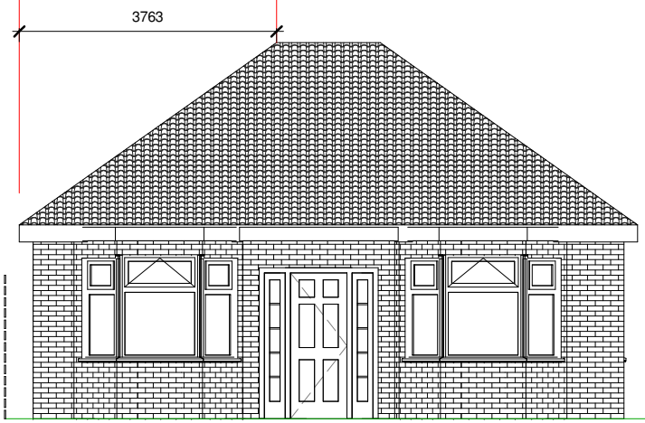
3 Front Elevation 1 : 100
