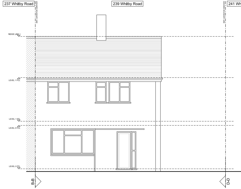
1. EXISTING FRONT ELEVATION A-A
