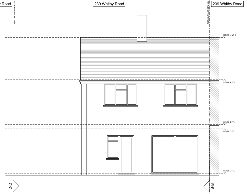
2. EXISTING REAR ELEVATION C-C
