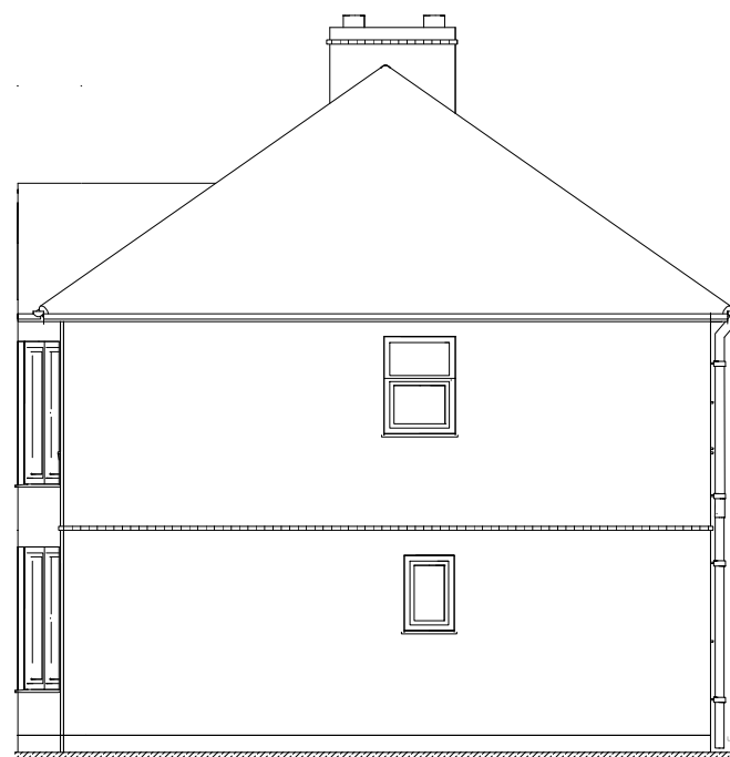
Right Side Elevation Plan 1:100
