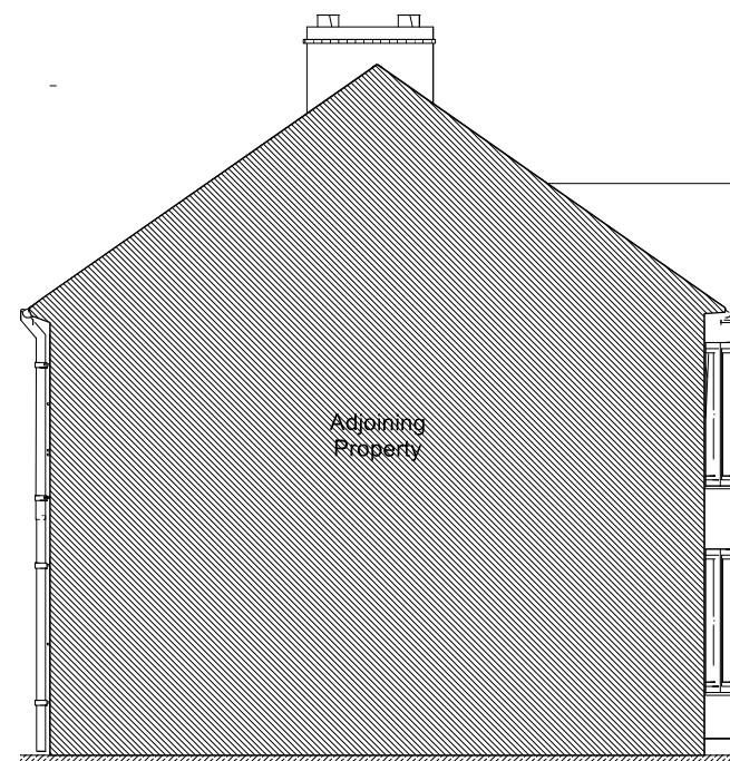
Left Side Elevation Plan 1:100
