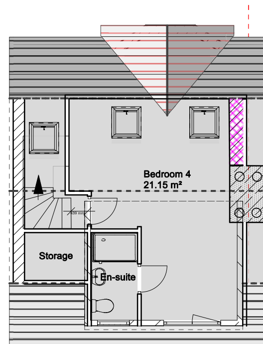
Proposed Loft Floor Plan 1:100
