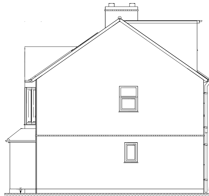
Proposed Right Side Elevation Plan 1:100
