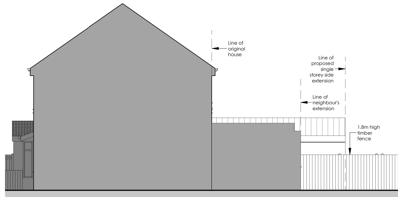
2 North Side Elevation (Proposed) 2310-A-302 1 : 100
