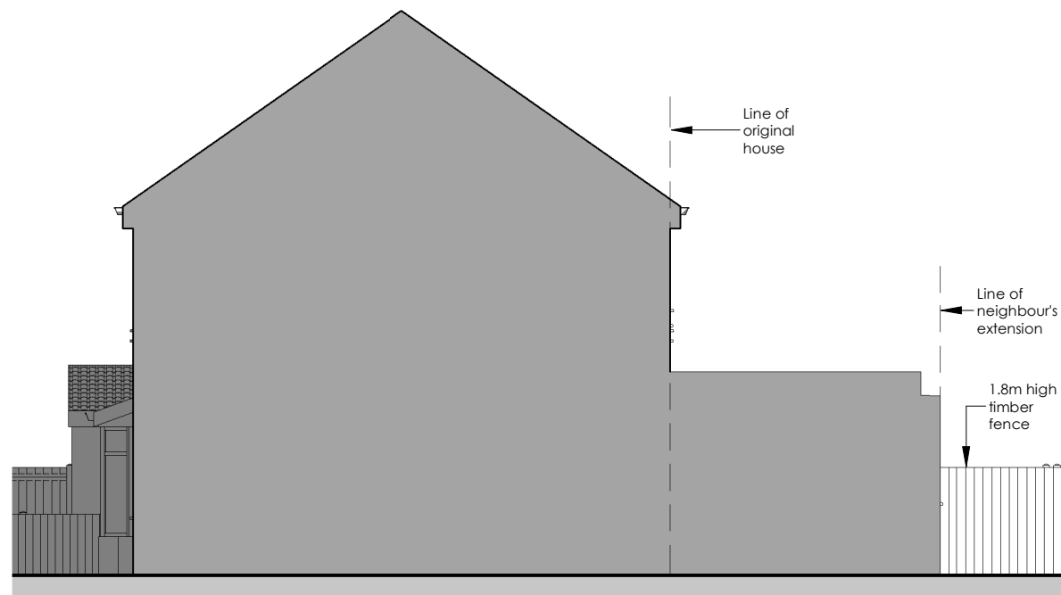
1 North Side Elevation (Existing) 2310-A-302 1 : 100
