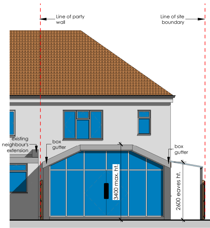
4 Rear Elevation (Proposed) 2310-A-301 1 : 100
