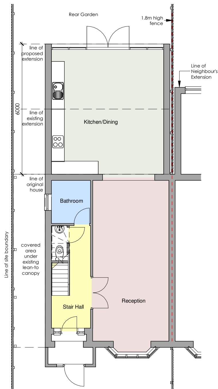
1 Ground Floor 2310-A-301 1 : 100
