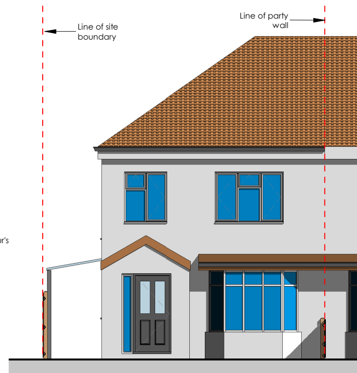
3 Front Elevation (Proposed) 2310-A-301 1 : 100
