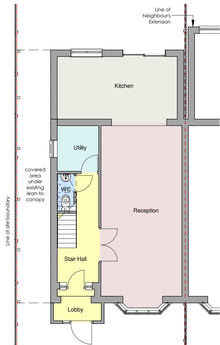
1 Ground Floor (Existing) 2310-A-200 1 : 100
