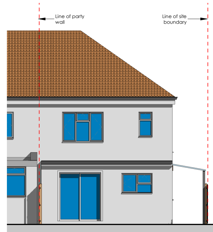
5 Rear Elevation (Existing) 2310-A-200 1 : 100
