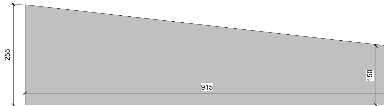
Detail D - Transition Kerb
