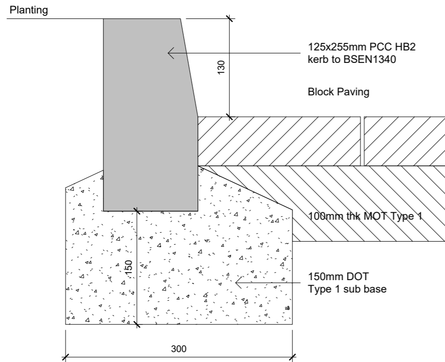
Detail E - Full Height Kerb
