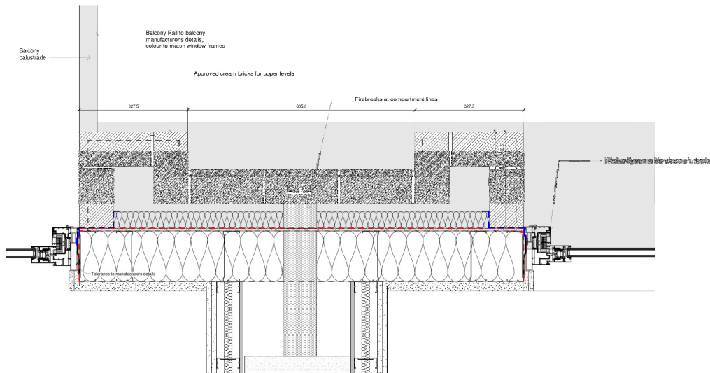
Second to Seventh Floor Façade/Brick Pier Detail
