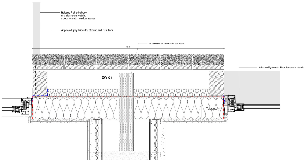
Ground to Second Floor Façade/Brick Pier Detail
