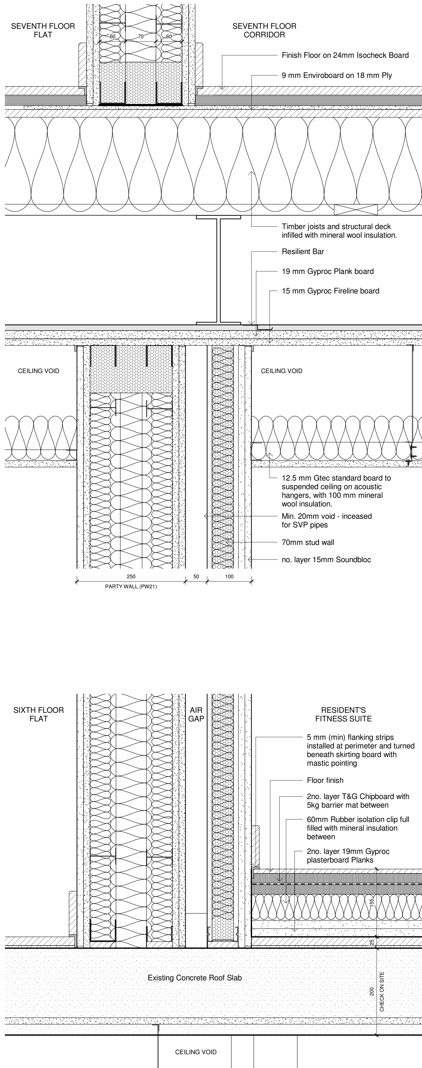
2 Fitness Suite Section - PW 23 1:5
