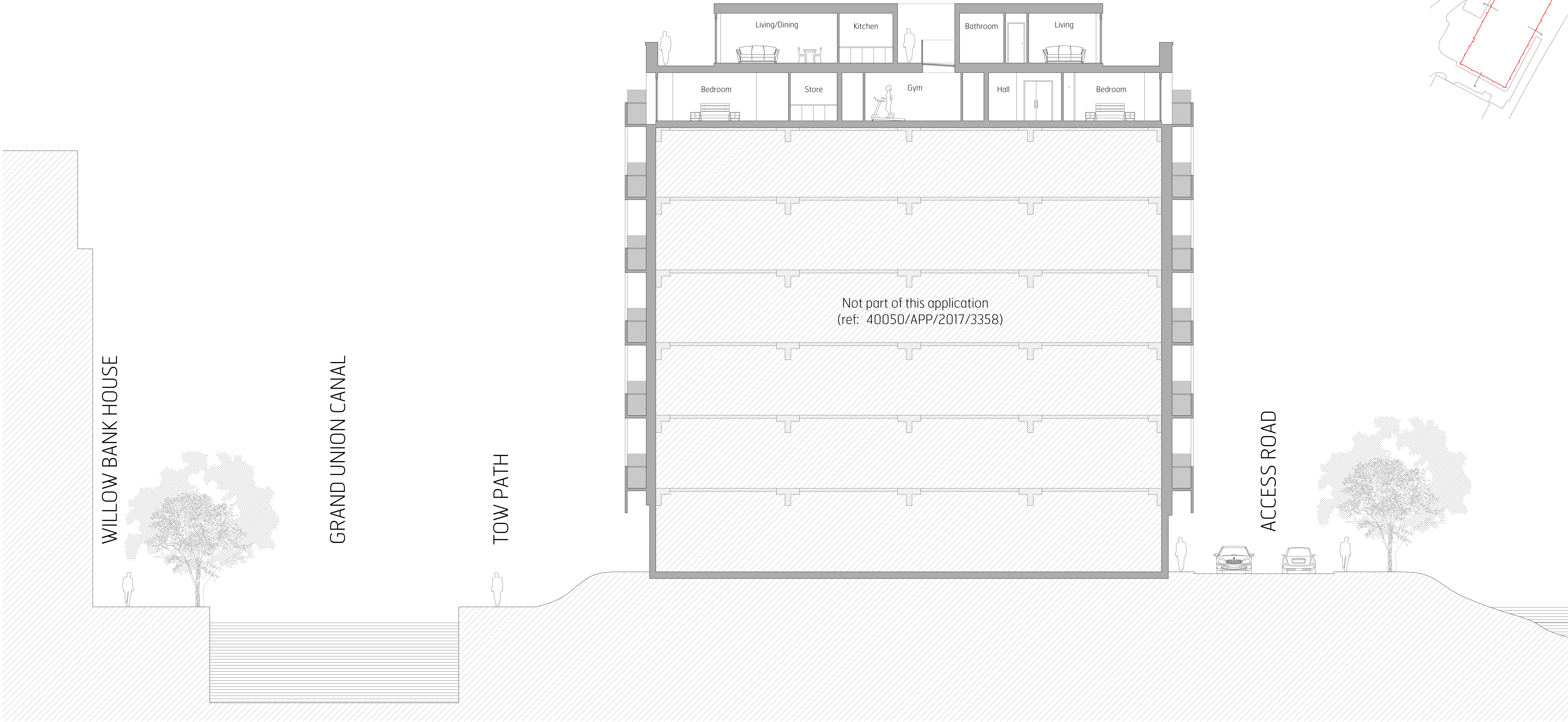
Proposed Section AA 1/100 @A1
