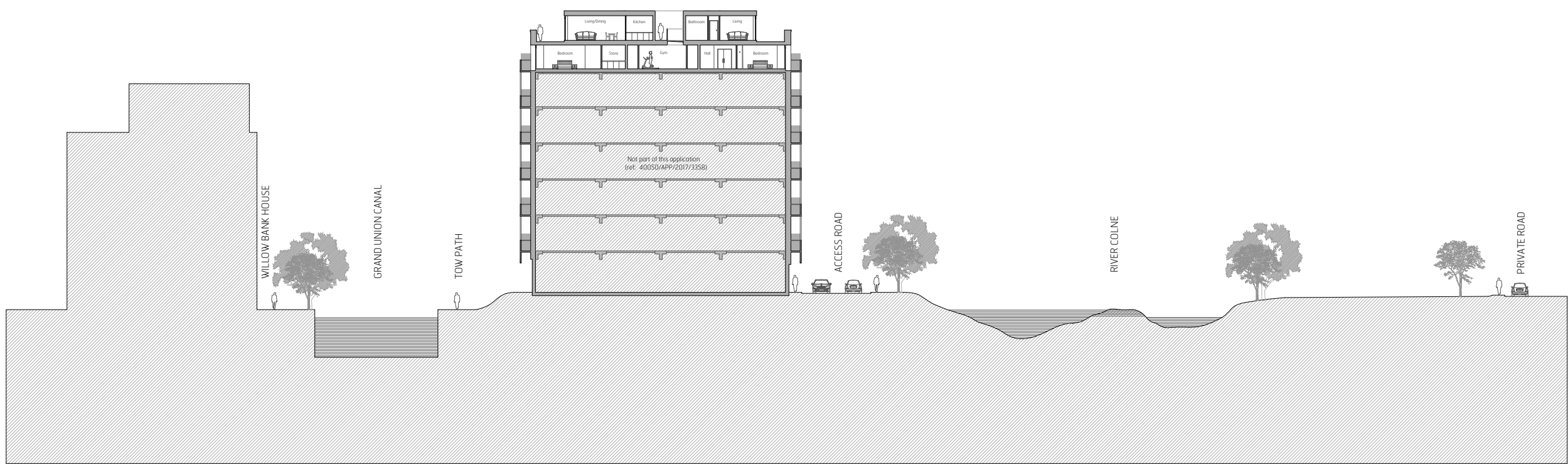
Proposed Roof Extension Section
