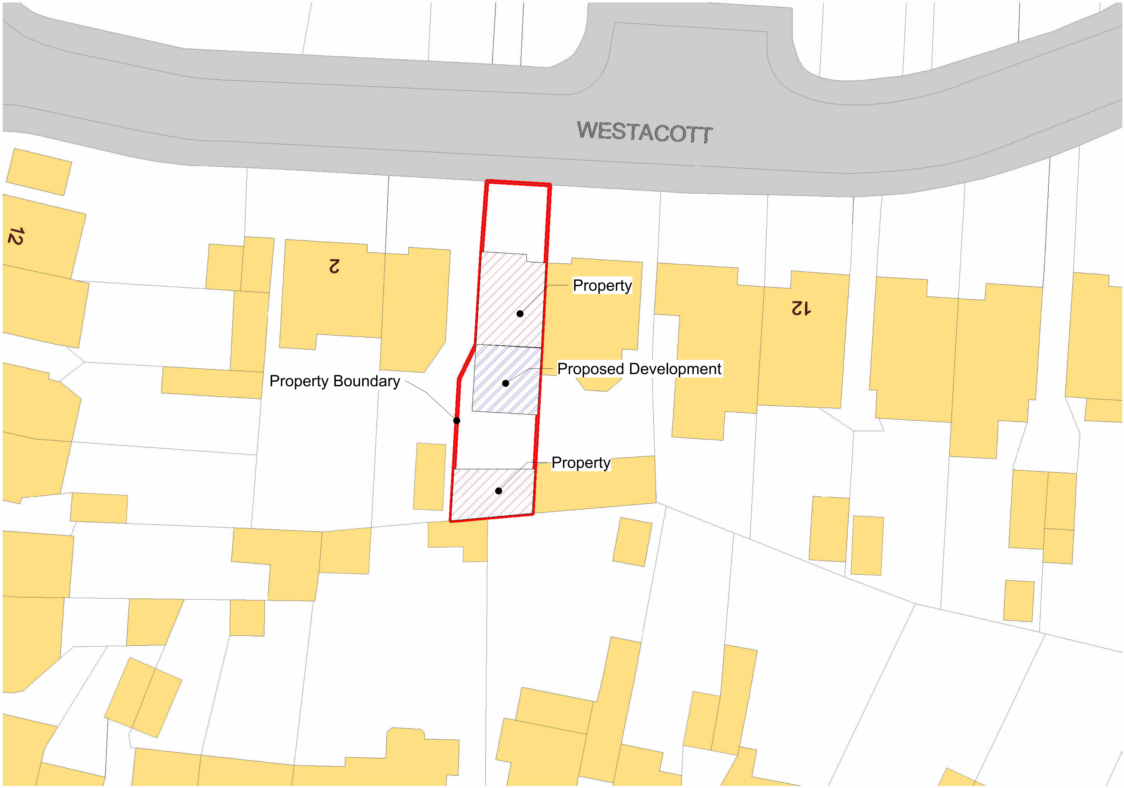
Location Plan, 1:200
