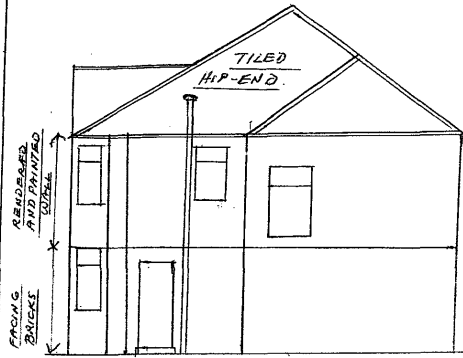
SOUTH EAST SIDE ELEVATION (AS EXISTING)
