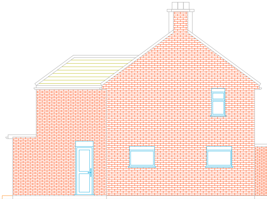
PROPOSED SIDE ELEVATION-2
