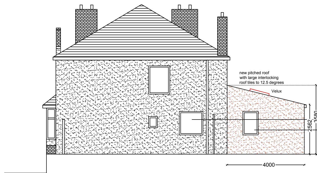
proposed side elevation from no.57 1:100
