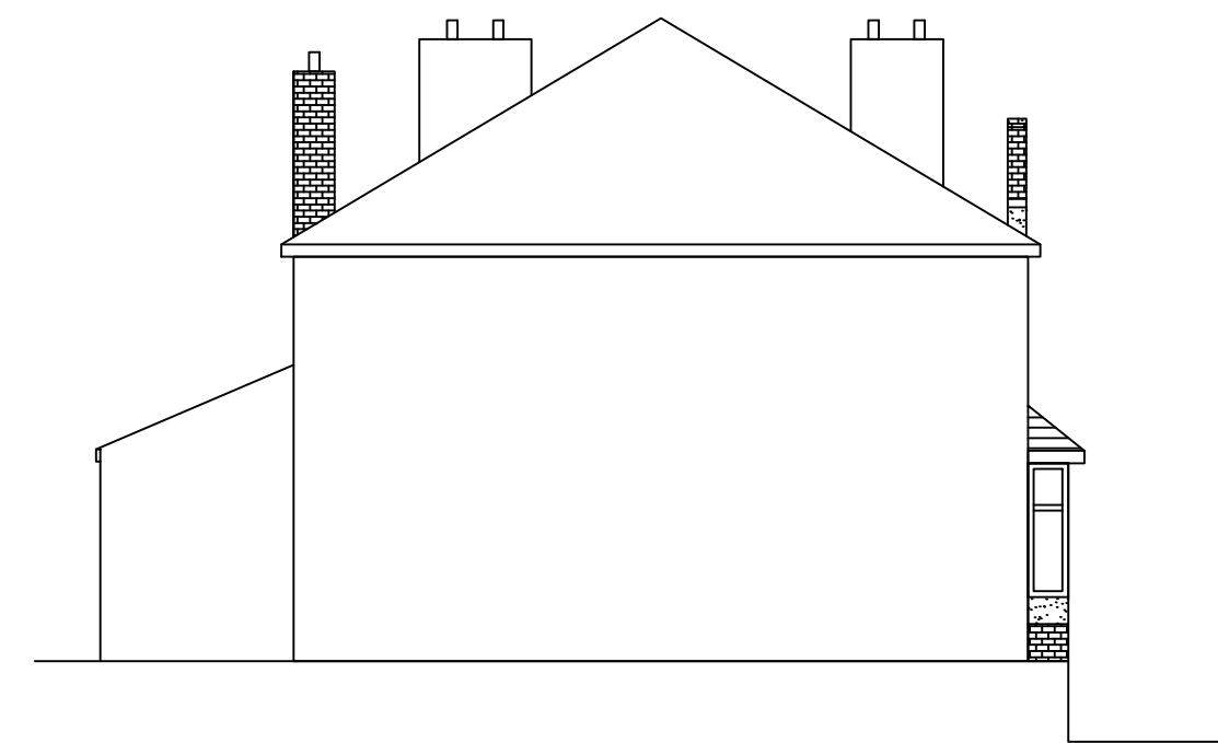
existing side elevation from no.53 1:100
