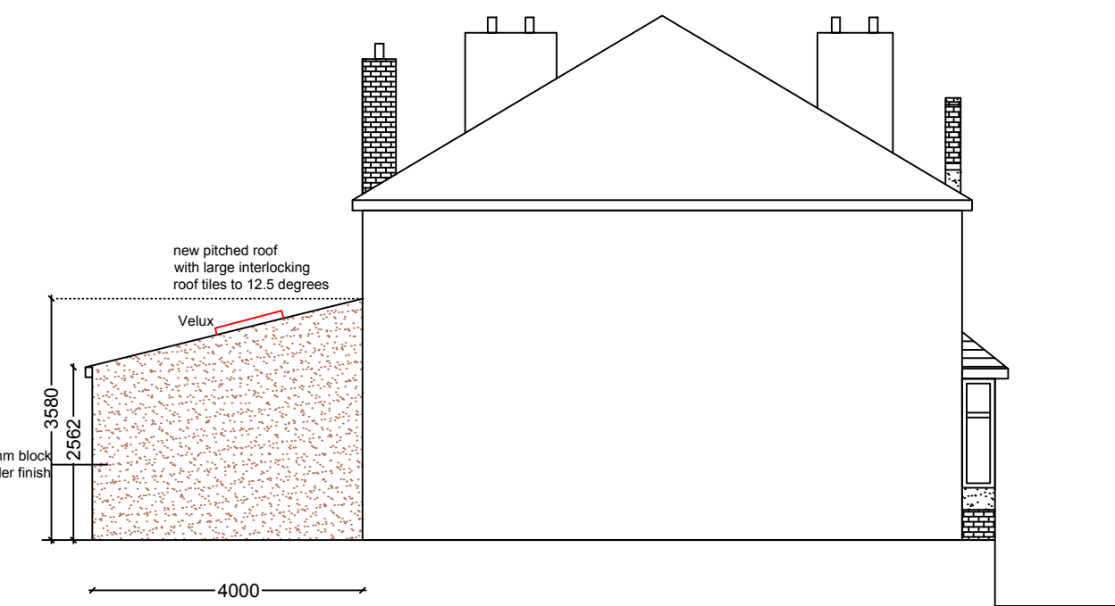
proposed side elevation from no.53 1:100
