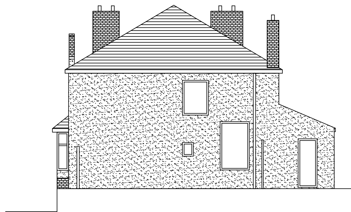
existing side elevation from no.57 1:100
