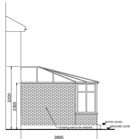
PROPOSED RIGHT ELEVATION (CONSERVATORY)
