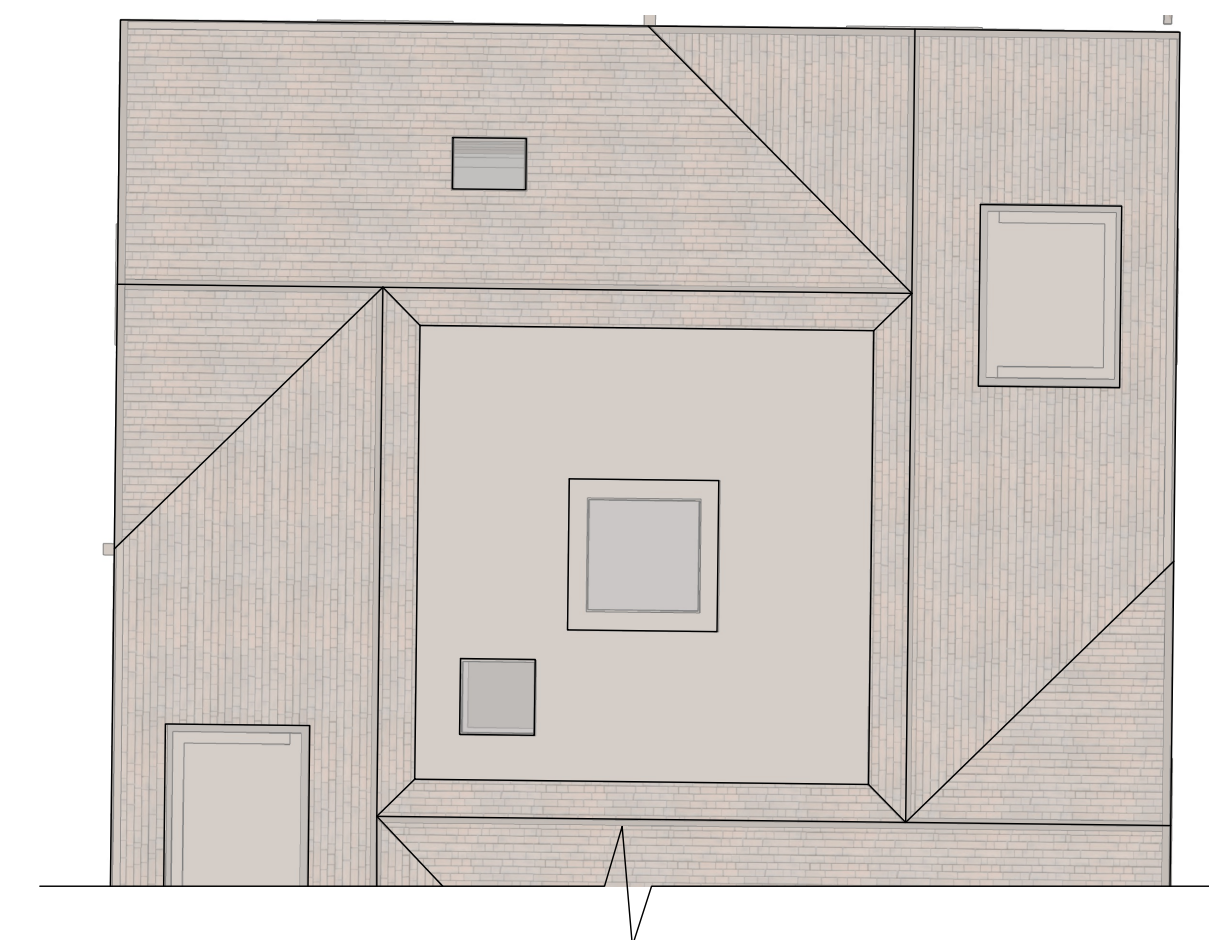
ROOF PLAN
