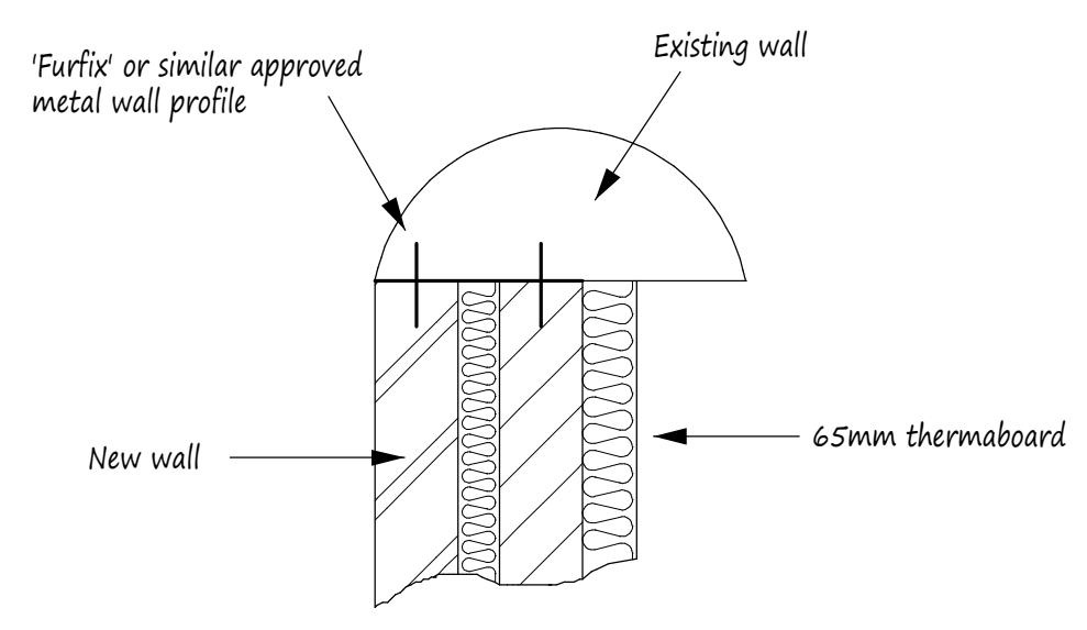
Detail - Where new wall abuts existing
