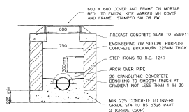
1200 x 750 BRICK MANHOLE Scale 1/20
