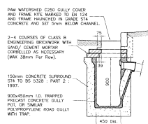
ROAD GULLY TYPICAL GULLY DETAILS (1/20)
