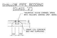
C250 CHANNEL DRAIN
