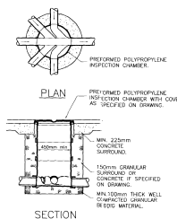
TYPICAL 450Ø (NOMINAL) POLYPROPYLENE INSPECTION CHAMBER DETAIL (500P SIMILAR) (1:20)
