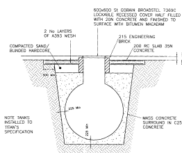
INSTALLATION FOR ENVIREAU 27,500 LITRE TANK SCALE 1:50
